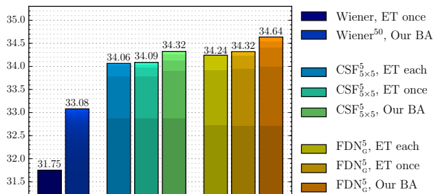
Figure 5: Comparison of boundary adjustment methods. Average PSNR (in dB) on the benchmark of Levin et al. with different boundary adjustment (BA) strategies. Vertical partitions of bars correspond to respective model stages. Our BA method shows a clear improvement over edgetapering (ET). See text for details.
